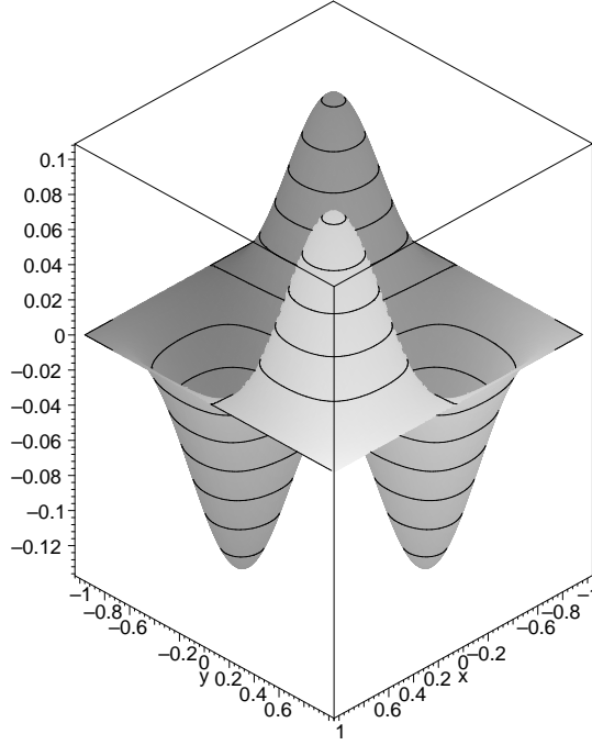
Figure 3: G_\lambda for \sqrt{\lambda} = 4.4 , between \sqrt{\lambda_1} = \pi and \sqrt{\lambda_2} \approx 4.49
