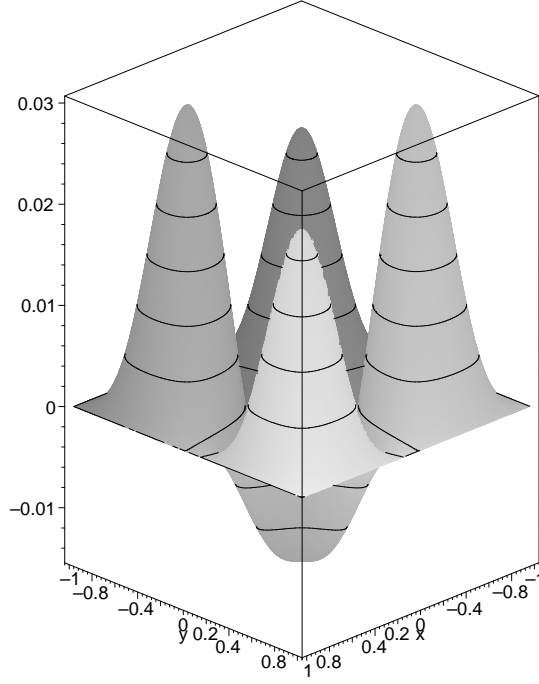
Figure 4: G_\lambda for \sqrt{\lambda} = 6 , between \sqrt{\lambda_2} \approx 4.49 and \sqrt{\lambda_3} = 2\pi
