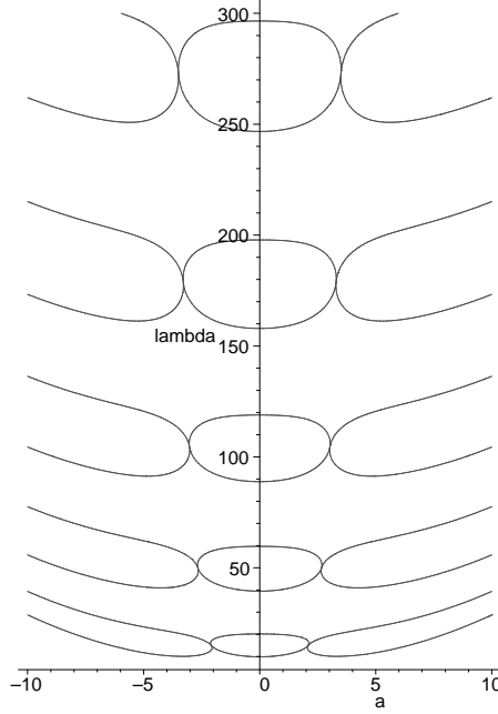
Figure 6: Eigenvalue curves and curves of sign change
