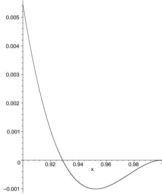
Figure 2: Looked at more closely
