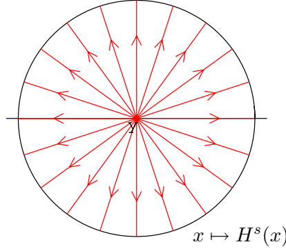
Figure 8: A conformal mapping changed H(x, y) to H^s(x) and, roughly spoken, put y in the center. Here is the result from Proposition 11: the function x \mapsto H^s(x) is radially increasing. The combination with Figure 7 and the inverse conformal mapping lead to Figure 1.
