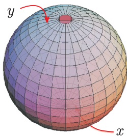
Figure 2: Sphere with a small hole near the north pole.
