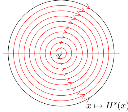
Figure 7: A conformal mapping changed H(x, y) to H^s(x) and put y in the center. By Proposition 9 the mapping x \mapsto H^s(x) is increasing to the right along all semicircles around 0.
