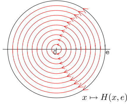
Figure 5: For y = e \in \partial B the function x \mapsto H(x, y) is increasing along semicircles to the left.
