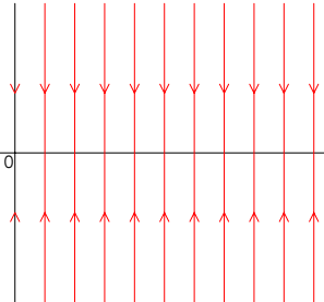
Figure 3: Illustration of Corollary 5; arrows denote increasing directions of X \mapsto \tilde{H}(X) .
