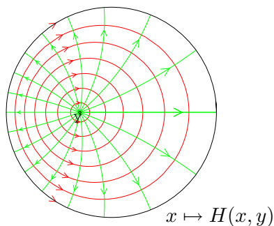
Figure 1: The geodesics through y in green (light) and the orthogonal trajectories in red (dark).
