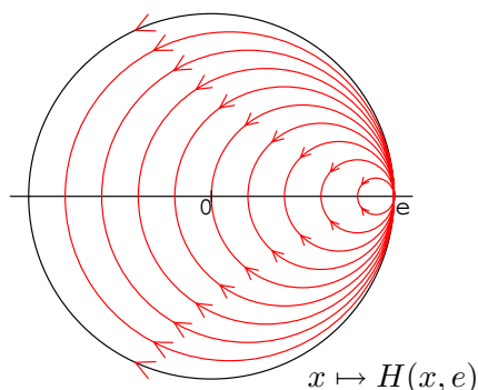
Figure 4: The result of Corollary 5 transformed back to the disk; arrows denote increasing directions of x \mapsto H(x, e) .
