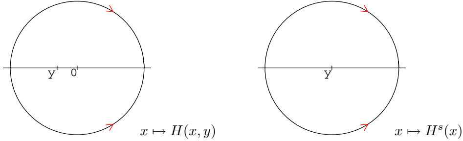
Figure 6: Using the symmetry between x and y we may conclude that for any y \in B , the function x \mapsto H(x, y) (left) is increasing along \partial B from the nearest boundary point of y to the most distant boundary point. Putting y = (-s, 0) with s > 0 it means increasing to the right along \partial B . Also the function x \mapsto H^s(x) (right) is increasing to the right along \partial B .
