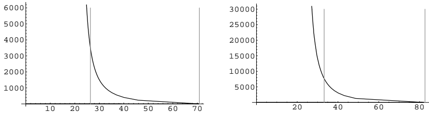
Second radial bifurcation branch for n = 6 and n = 7
