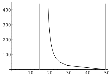
Second radial bifurcation branch \lambda \mapsto \omega(\lambda) = u(0) for n = 4
