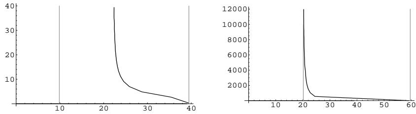
Second radial bifurcation branch for n = 3 and n = 5
